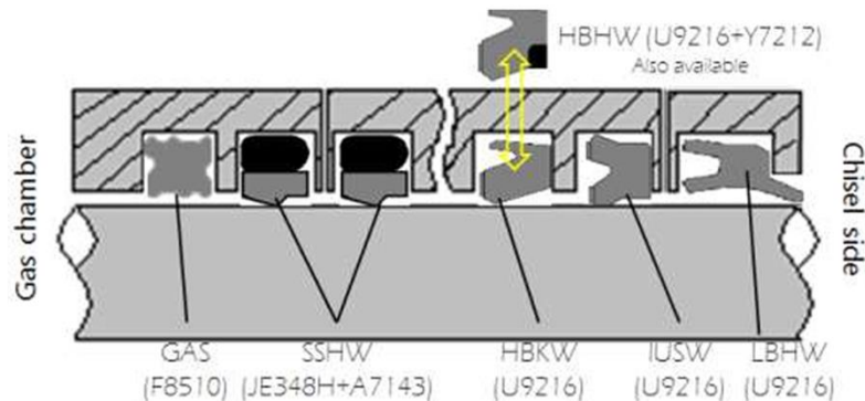
Hydraulic breaker
